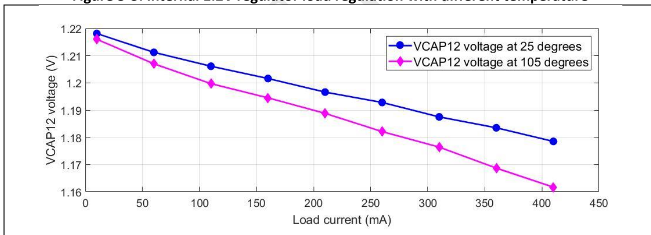
Figure 5-3: Internal 1.2V regulator load regulation with different temperature
