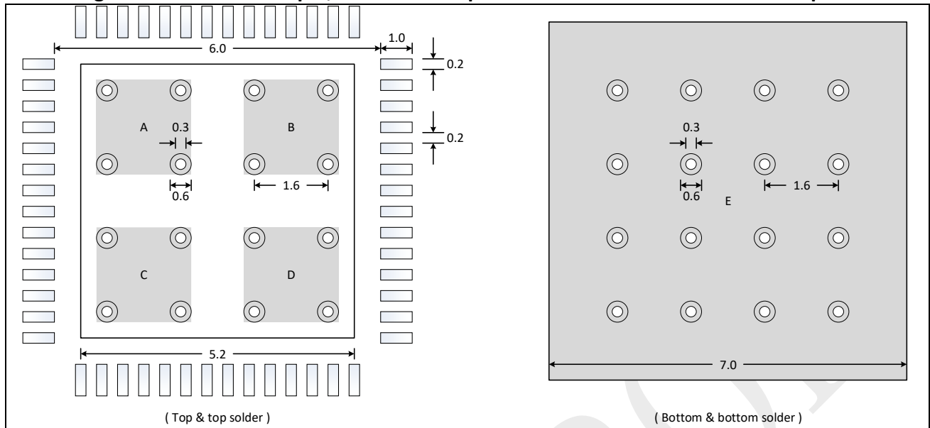
Figure 7-2: QFN56 – 56 pin, 7mm x 7mm quad flat no-lead recommended footprint
