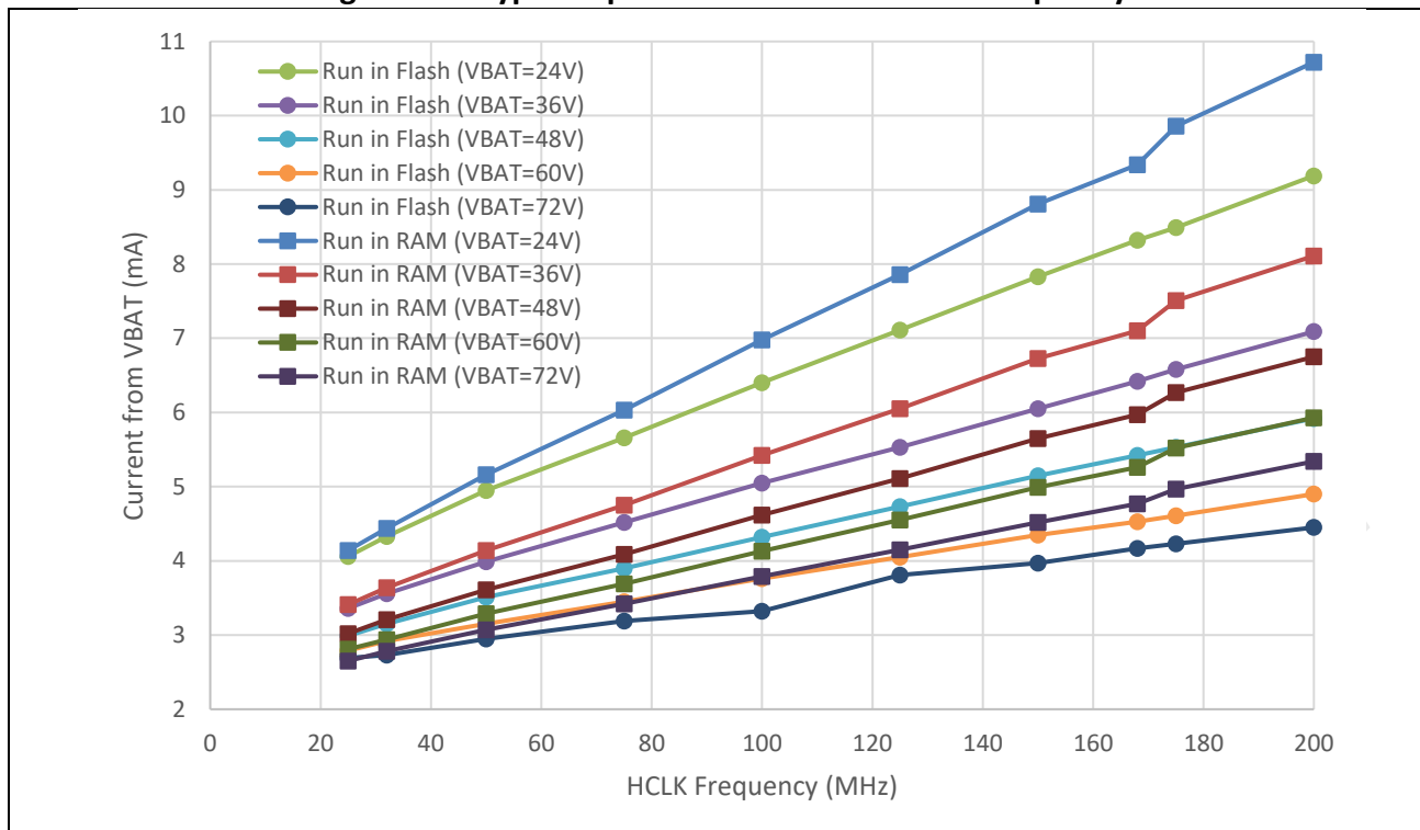
Figure 5-1: Typical operational current versus frequency
