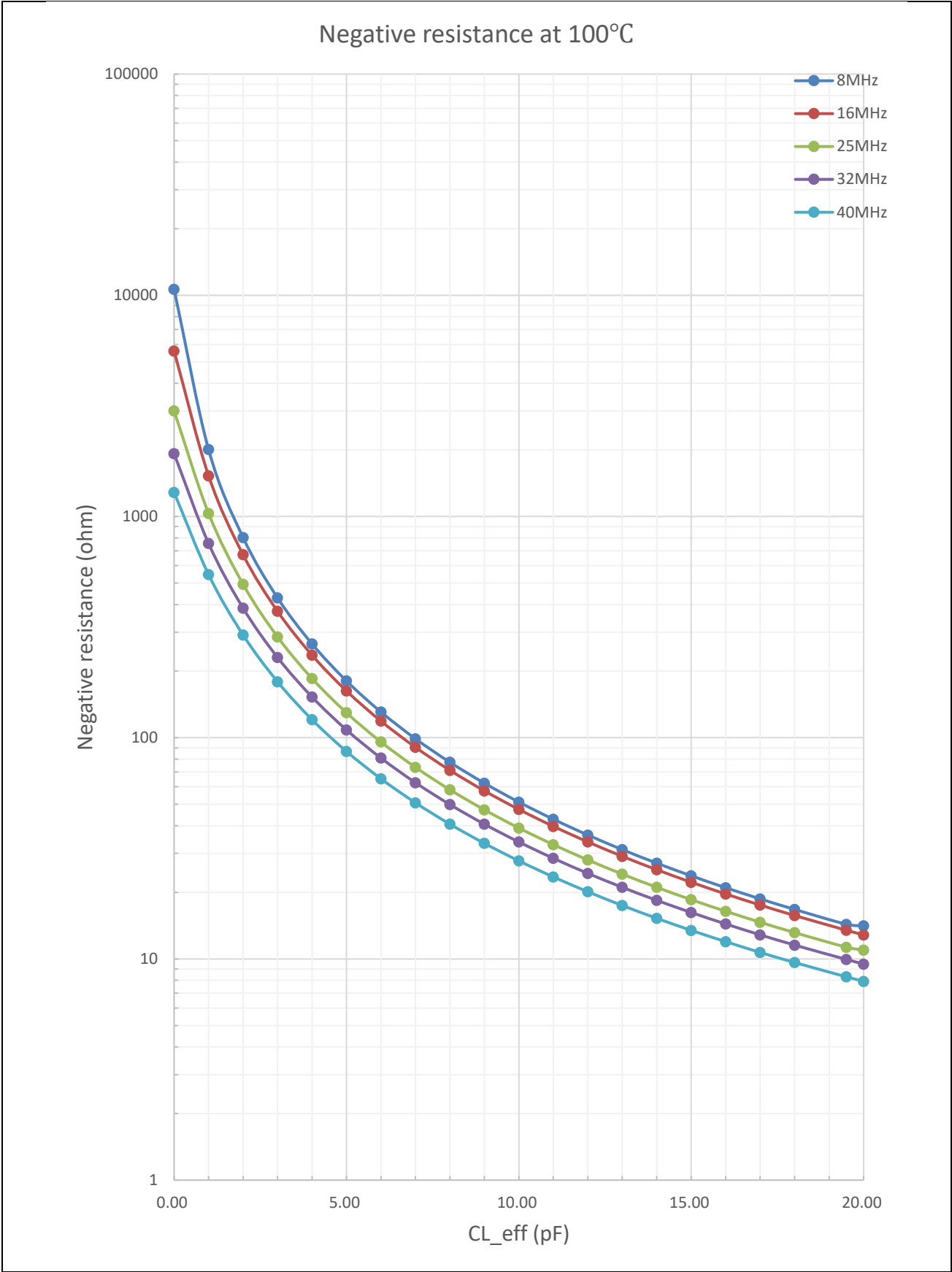
Figure 5-6: The negative resistance of the on-chip crystal oscillator at 100 °C
