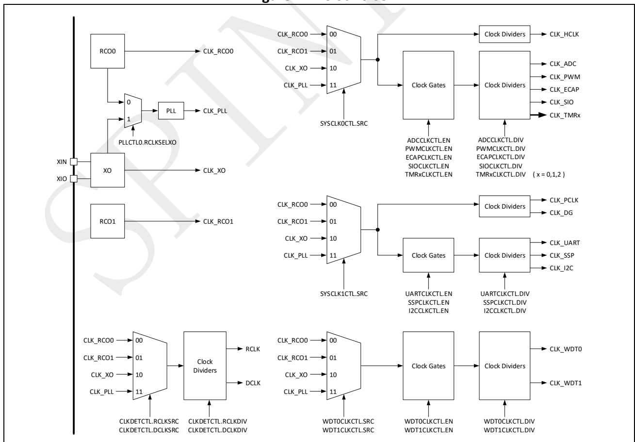
Figure 2-1: Clock tree
